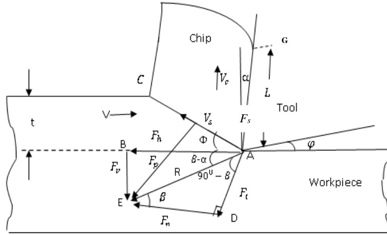
Fig. 2: Cutting forces components in orthogonal cutting (Juneja et al. , 2003)
