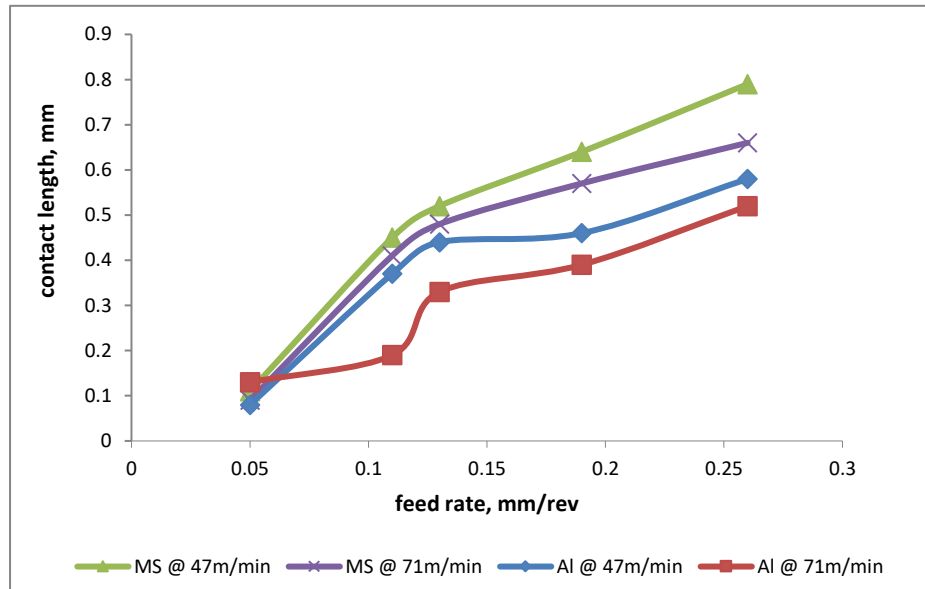
Fig. 3: Effect of tool-chip contact length and feed on aluminium and mild steel at a depth of cut, 0.10m and constant speeds V= 47\text{m/min} and 71\text{m/min}
