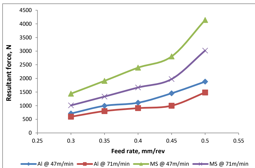
Fig. 6: Effect of feed on the resultant forces of aluminum and mild steel at a depth of cut, 0.10m and constant speeds, V=47\text{m/min} and 71\text{m/min}
