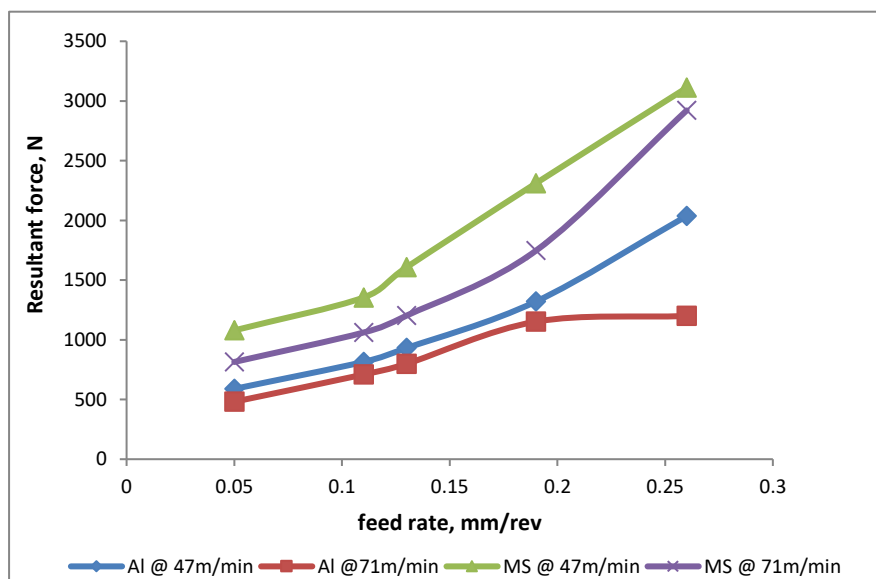
Fig. 5: Effect of feed on the resultant forces of aluminum and mild steel at a depth of cut, 0.10mm and constant speeds, V=47\text{m/min} and 71\text{m/min}
