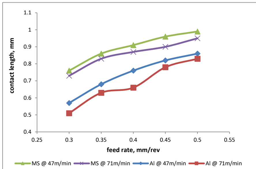
Fig. 4: Effect of tool-chip contact length and feed on aluminium and mild steel at a depth of cut, 0.20mm and constant speeds, V=47\text{m/min} and 71\text{m/min}
