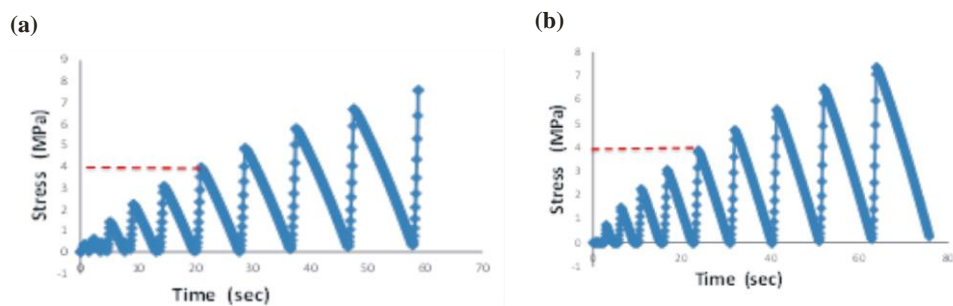
Figure 3.6: MSCR Test Result for Stress versus experimental time for Microhybrid Cured with (a) LED and (b) HiLED
