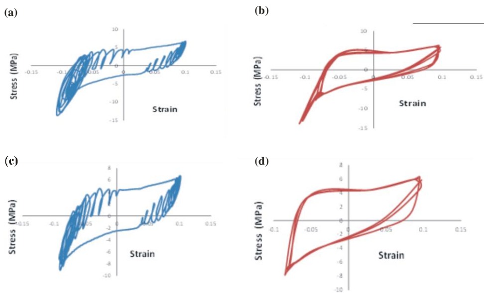
Figure 3.4: (a) One cycle of uniaxial loading and unloading of Microhybrid cured with LED (b) Several cycles of uniaxial loading and unloading of Microhybrid cured with LED (c) One cycle of uniaxial loading and unloading of Microhybrid cured with HiLED (d) Several cycles of uniaxial loading and unloading of Microhybrid cured with HiLED
