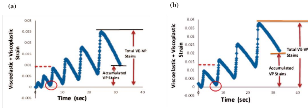
Figure 3.7: MSCR Test Result for Total Strain versus experimental time for Nanofilled cured with (a) LED and (b) HiLED
