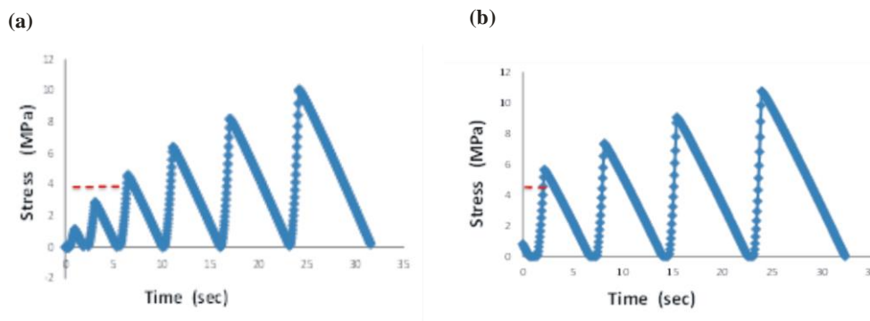
Figure 3.8: MSCR Test Result for Stress versus experimental time for Nanofilled Cured with (a) LED and (b) HiLED
