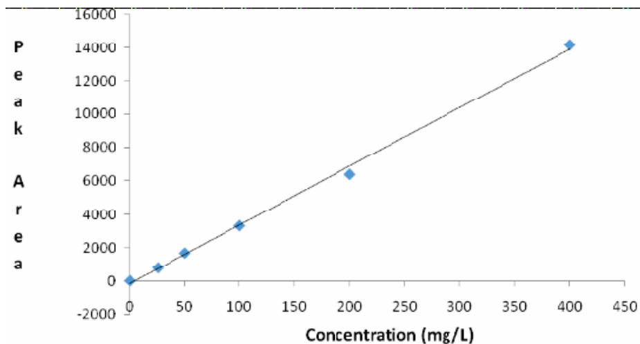
Figure 6: Linearity and range of Sulphamethoxazole (SMZ)
